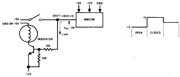
FIGURE 2. Shift Logic I/O Interface
