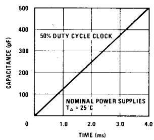
FIGURE 1. Key-Bounce Mask Time
